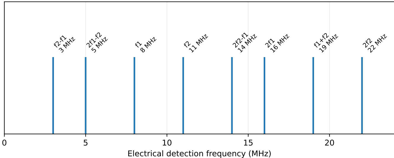
Illustrative low-order output channels for f_1 = 8 MHz, f_2 = 11 MHz
