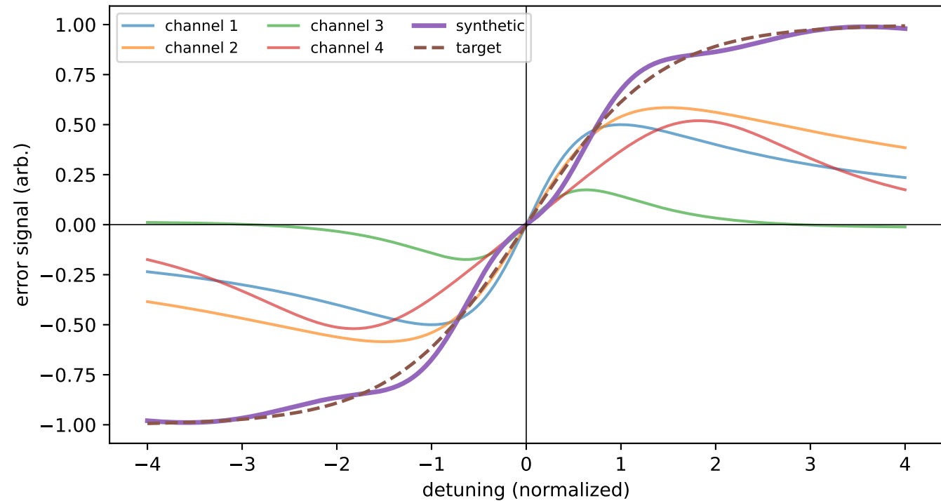
Toy illustration: channel diversity enables discriminator-shape synthesis
