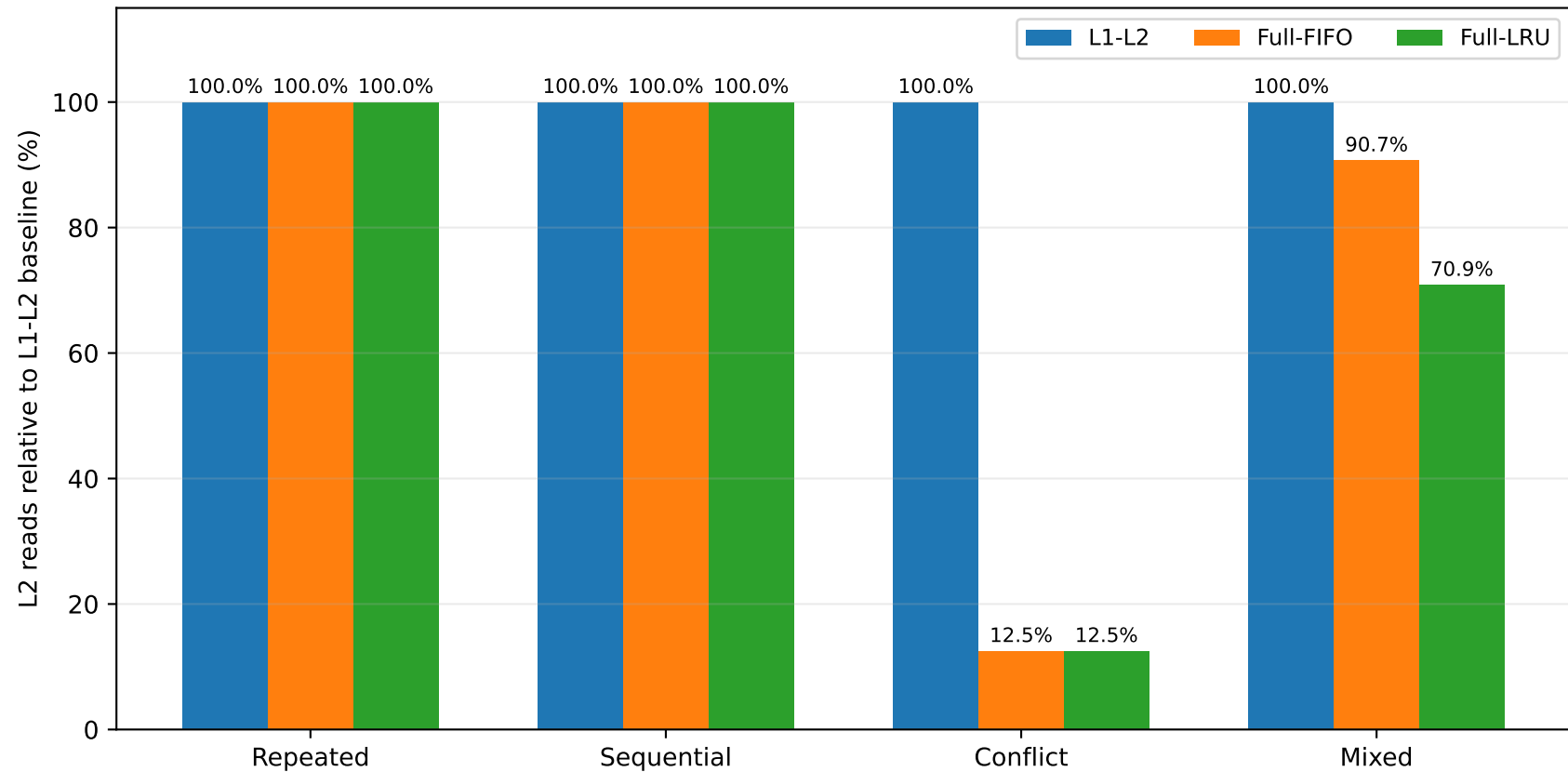
Reduction of L2 traffic
