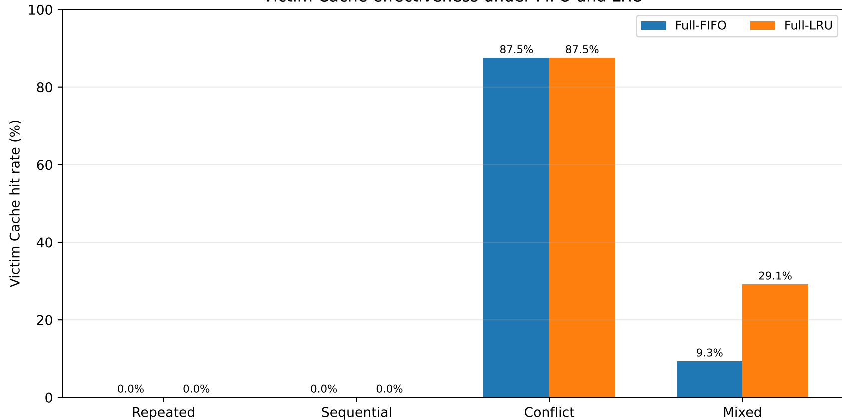
Victim Cache effectiveness under FIFO and LRU
