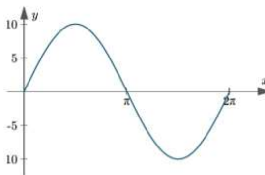
The graph of y = 10 \sin(x) for 0 \leq x \leq 2\pi
