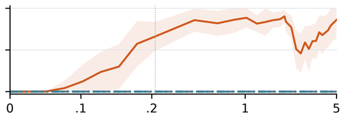
MultiRoom-N6
