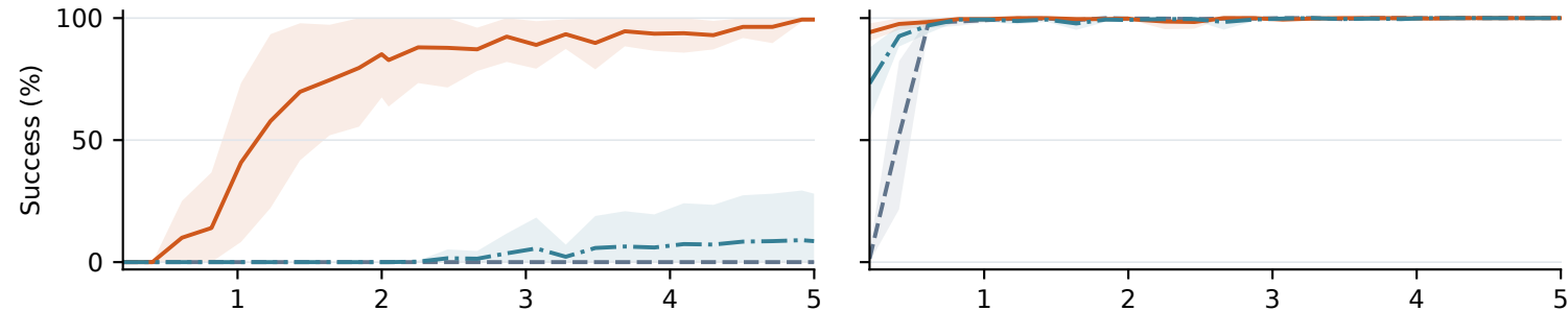
KeyCorridor-S3R3 / PPO
