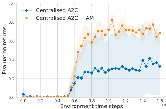
(b) Centralized A2C with and without representation-based agent models.
