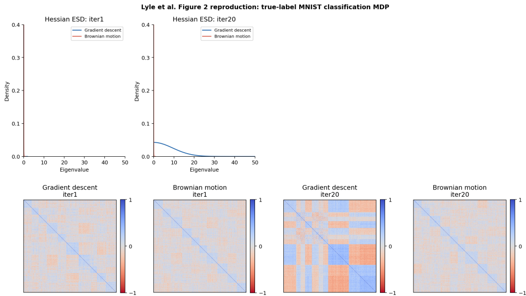
Figure 4: Hessian spectra and gradient covariance matrices are computed using the probe loss. For the gradient covariance heatmaps, the color scale is set to [-1, 1] because the entries are cosine similarities.
