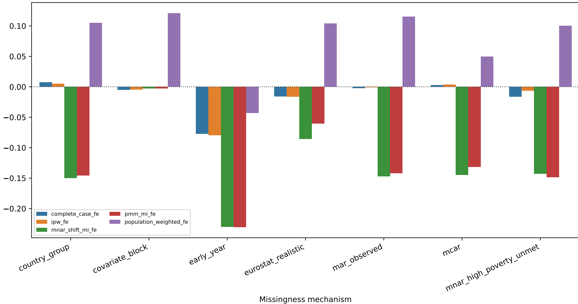
Mean bias relative to reference estimand
