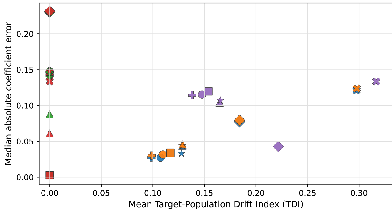
Target drift and coefficient error by mechanism-estimator cell
