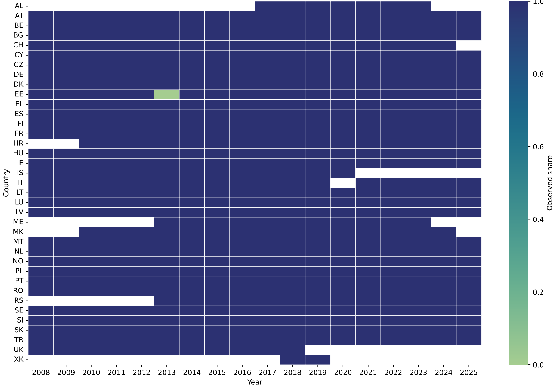
Missingness coverage: Population weights
