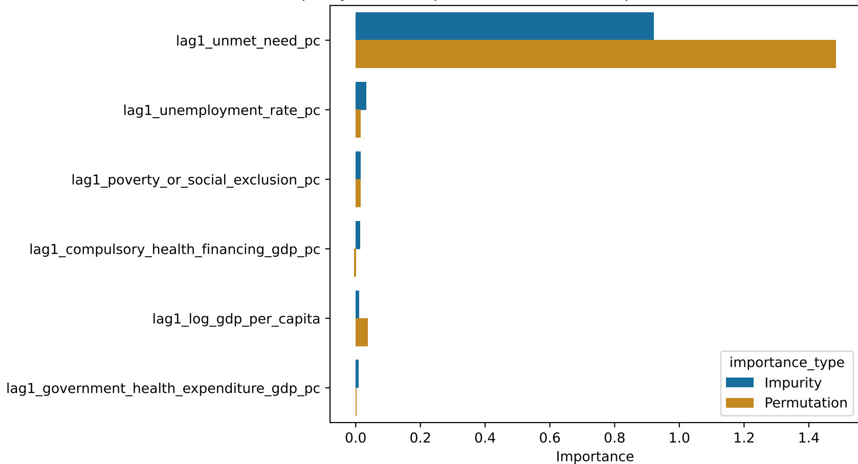
Impurity-based vs permutation feature importance, best tree model, tes
