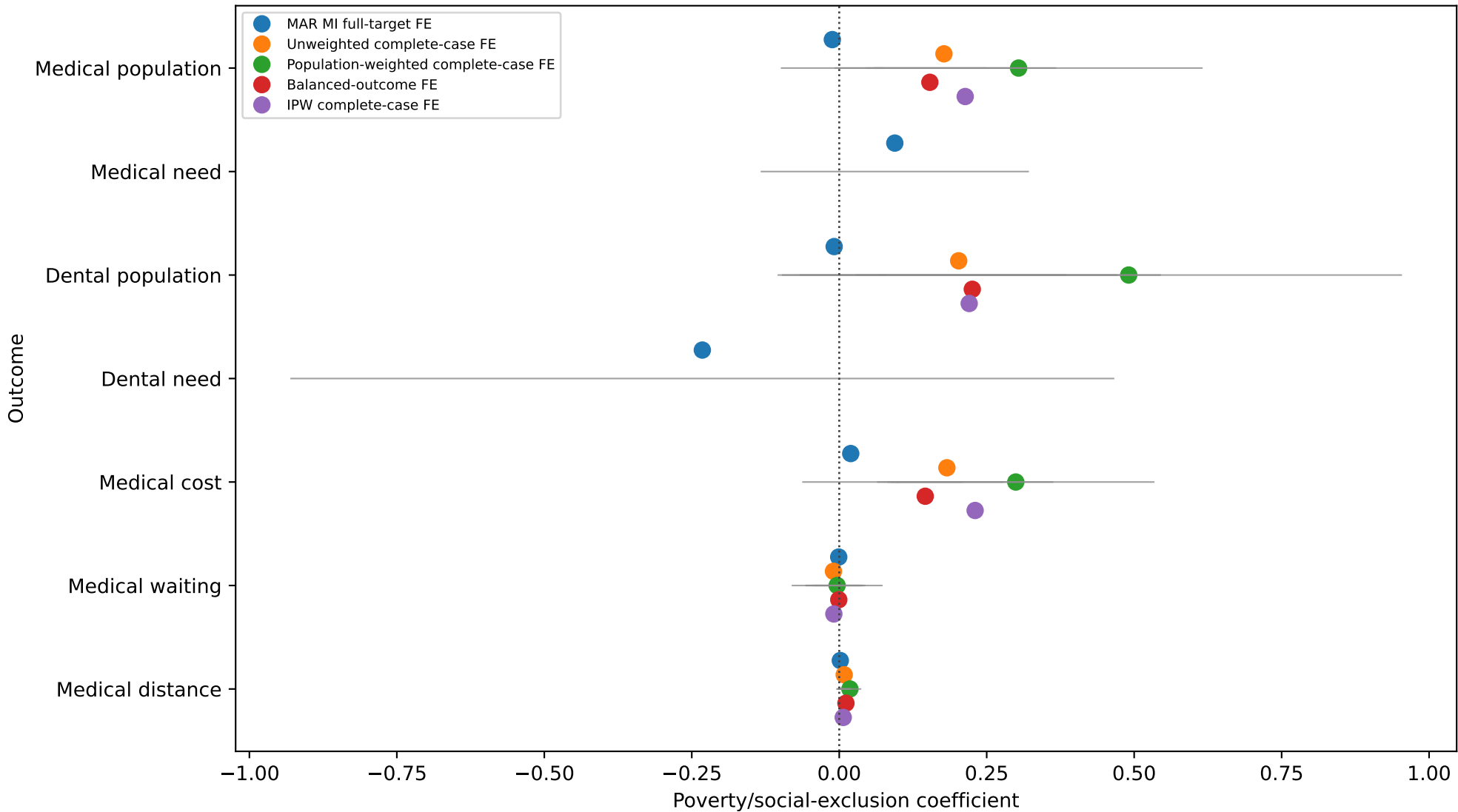
Outcome-by-estimator coefficient stability
