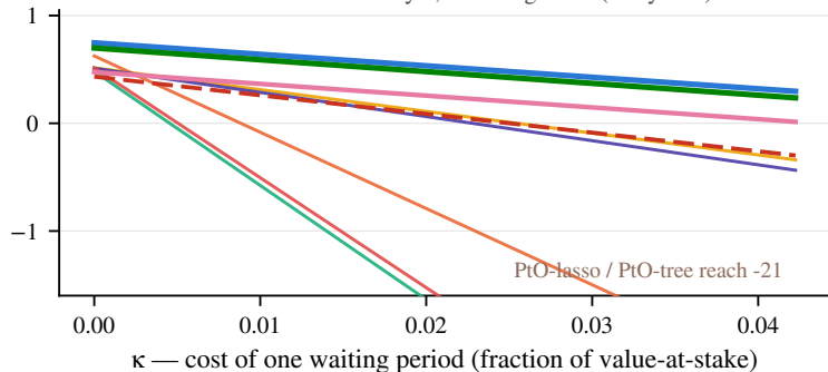
(a) DAPV( \kappa ) averaged over all 6 datasets
