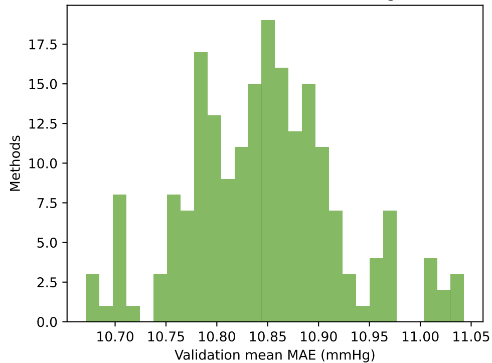
Locked 200-method screening
