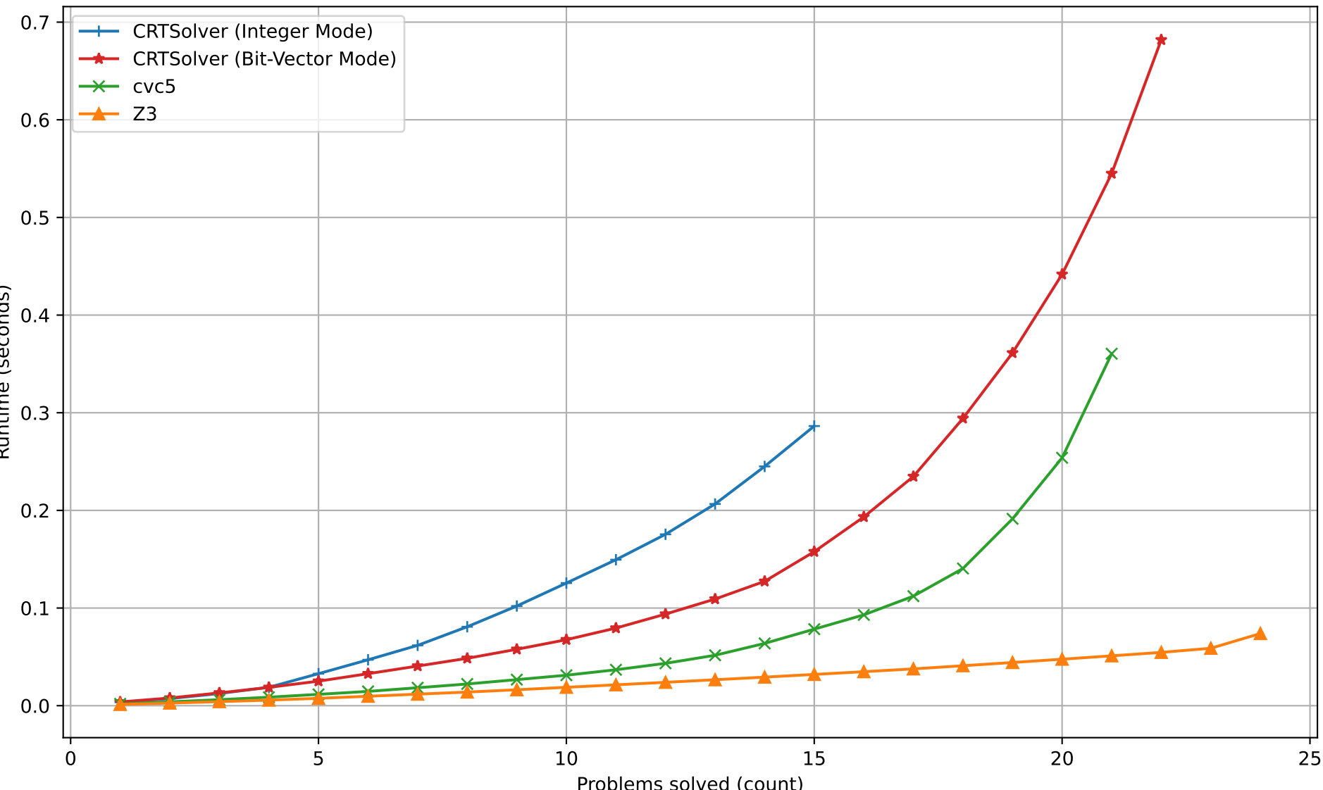
Speed of SMT Solvers with Non-Linear Integer Equations (4GB, 0.1s)
