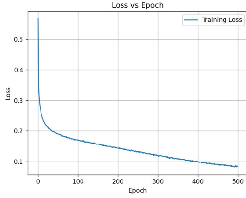
(a) Hybrid Model Loss vs Epoch
