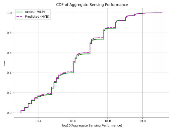
(a) Hybrid Model's CDF vs Sensing Performance
