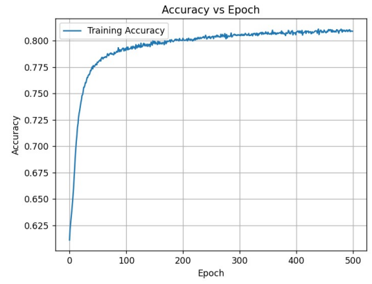
(b) CNN Model Accuracy vs Epoch
