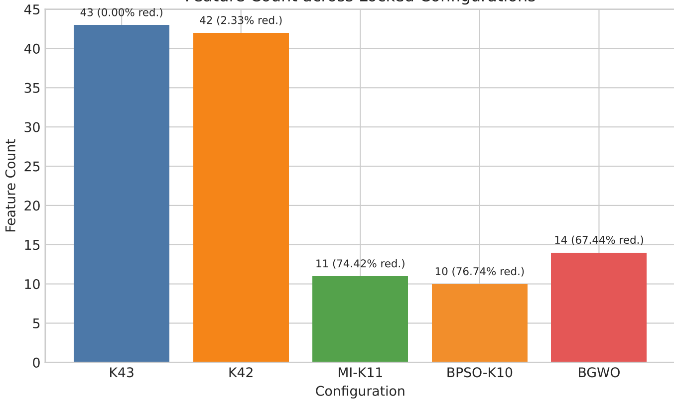
Feature Count across Locked Configurations
