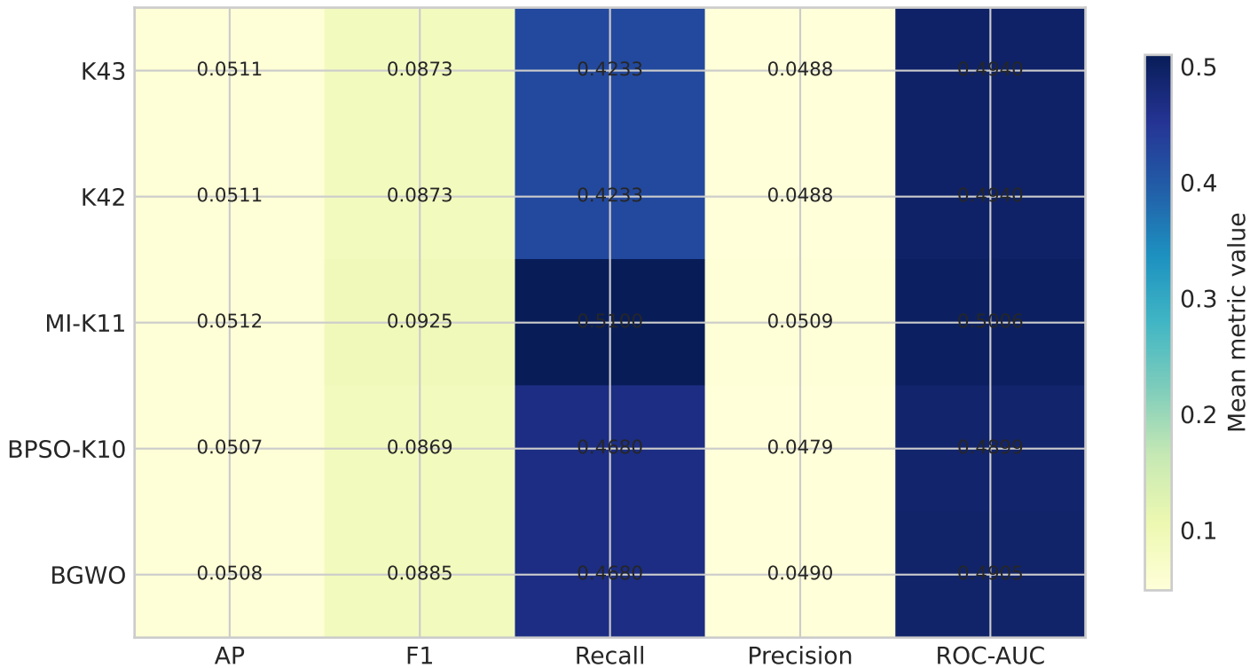
Logistic Regression Final-Test Mean Metrics (V0.9-E)
