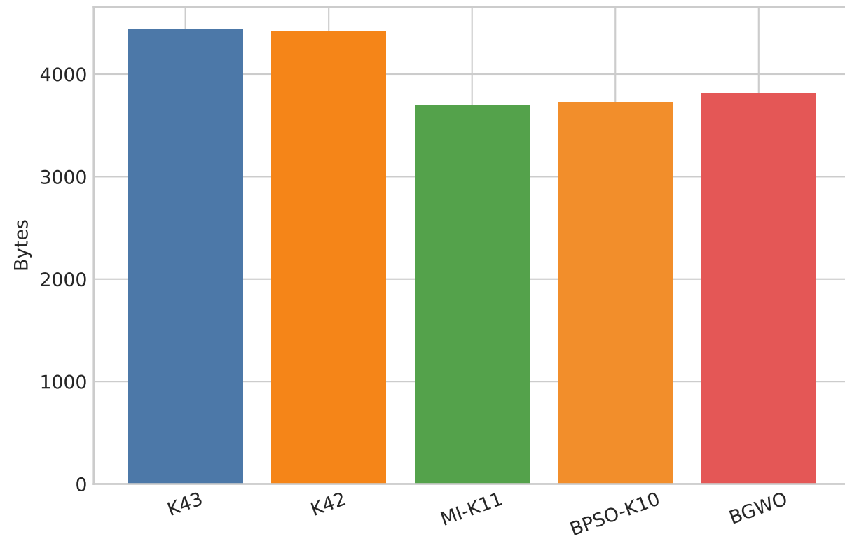
Decision Tree Serialized Model Size
