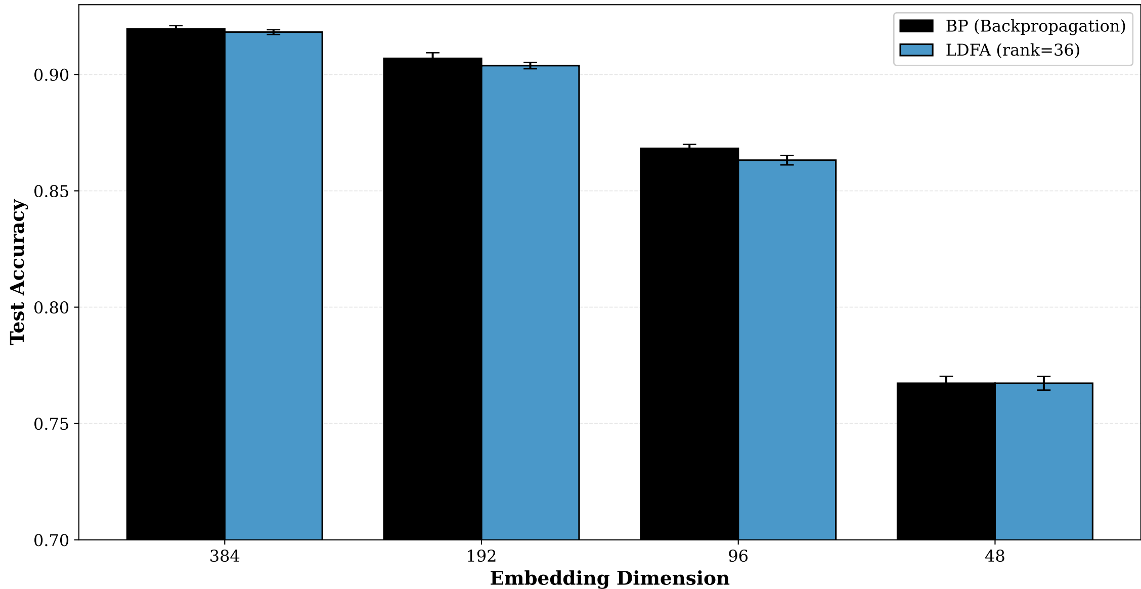
BP vs LDFA Performance Across Embedding Dimensions (CIFAR-10, ViT-B/16)
