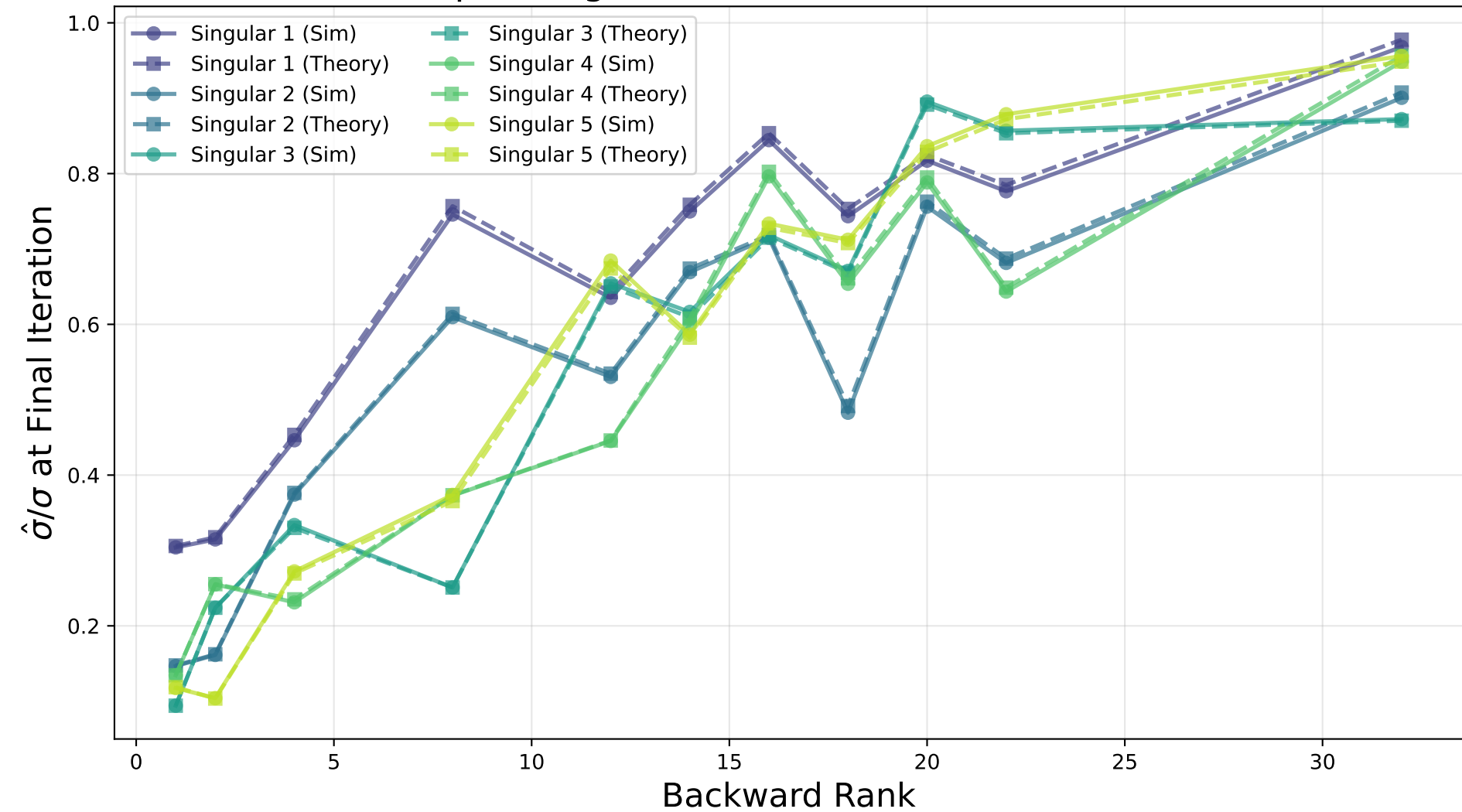
Top 5 Singular Values vs Backward Rank
