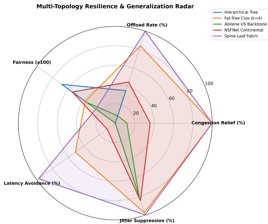
Figure 7.2: Radar chart depicting resilience metrics across topologies under stress testing.
