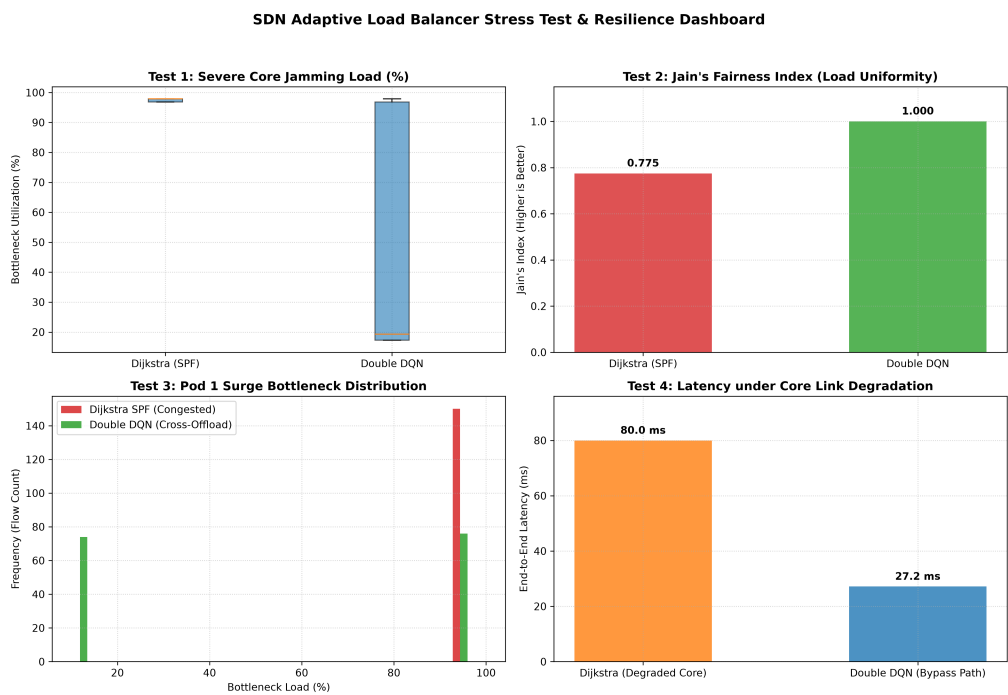
Figure 7.3: Load balancing stress test showing real-time utilization equalization under traffic surges.
