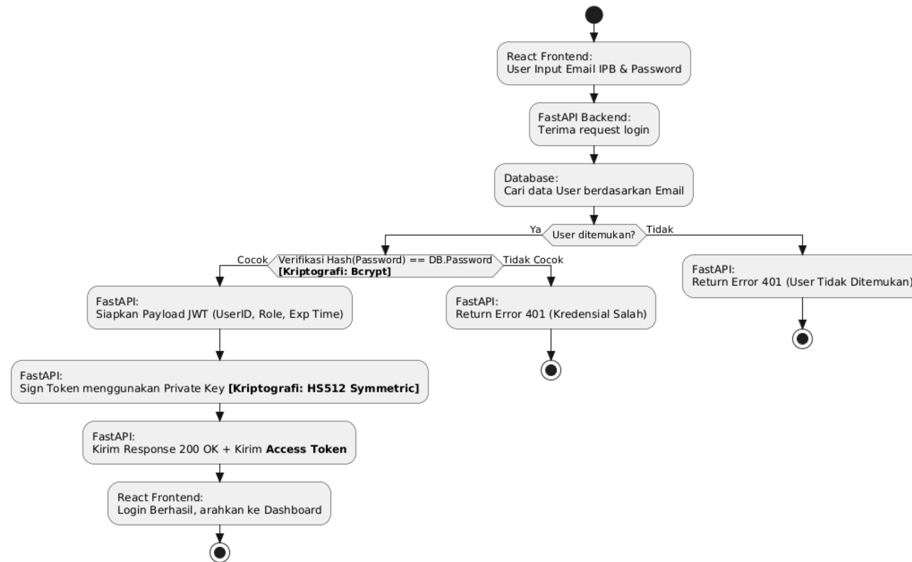
Diagram Alur Authentication (Login & Generate JWT)
