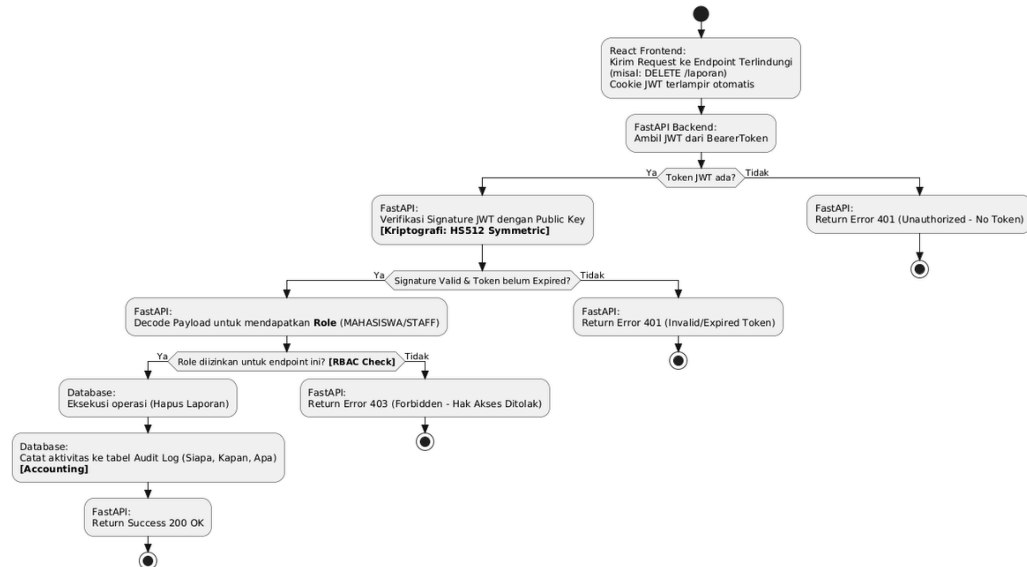
Diagram Alur Authorization & Accounting (Akses Resource)
