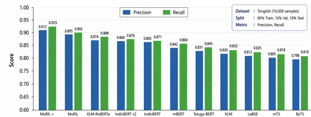
Fig. 4. Precision vs Recall comparison
