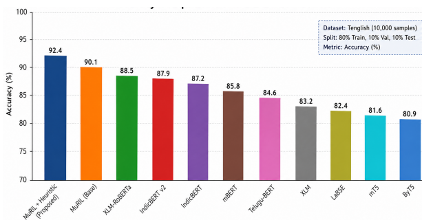
Fig. 2. Accuracy comparison across transformer models
