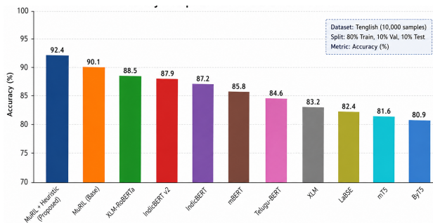
Fig. 2. Accuracy comparison across transformer models
