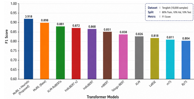
Fig. 3. F1 score comparison across models
