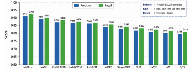
Fig. 4. Precision vs Recall comparison
