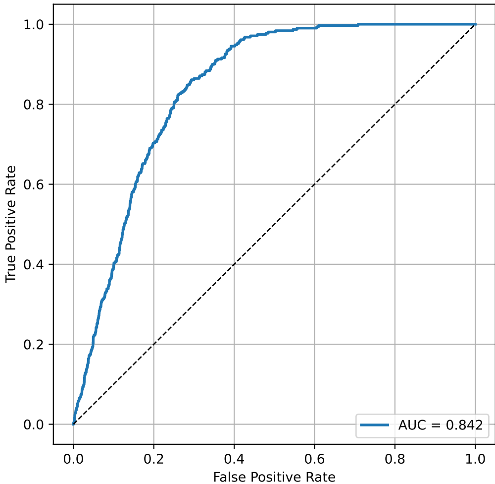
ROC (max cosine distance)
