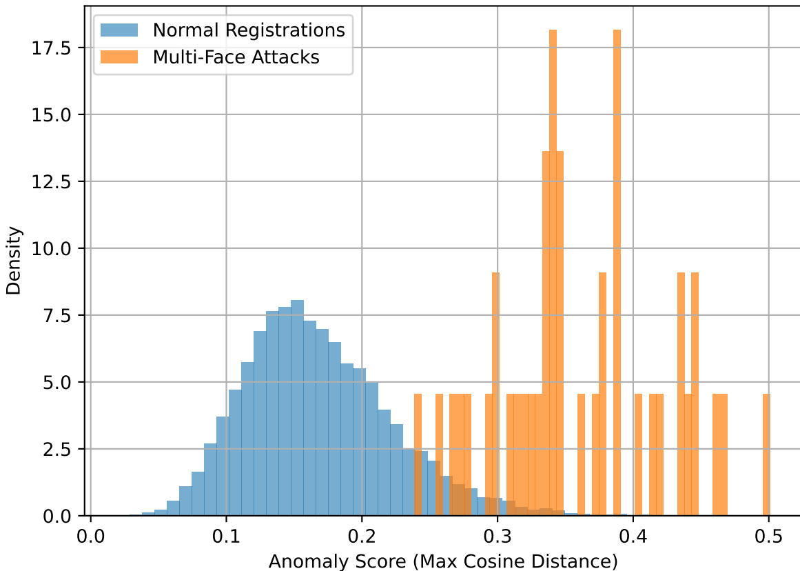
Score Distribution: Normal vs Multi-Face Registration Attacks
