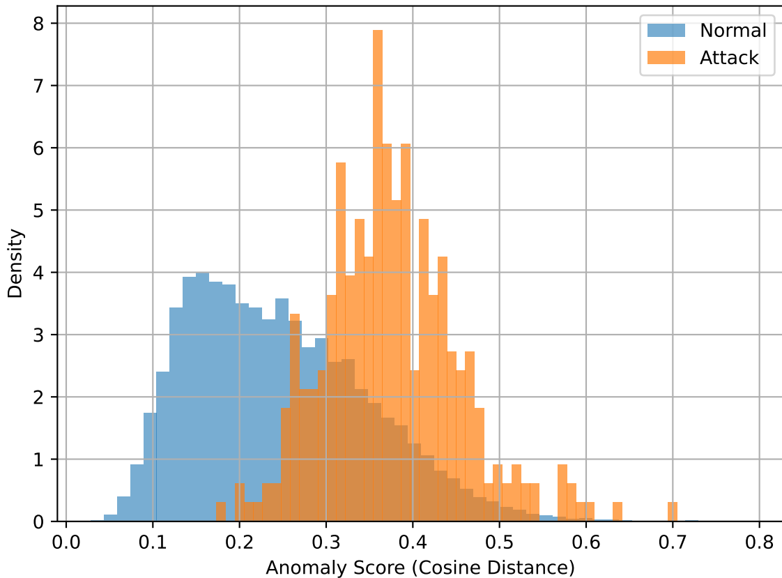
Score Distribution (max cosine distance)
