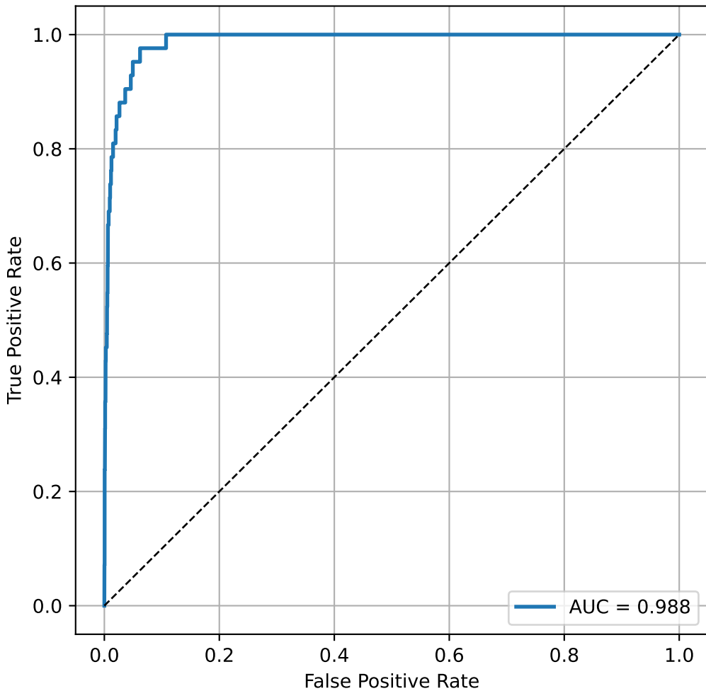
ROC: Multi-Face Registration Attack Detection
