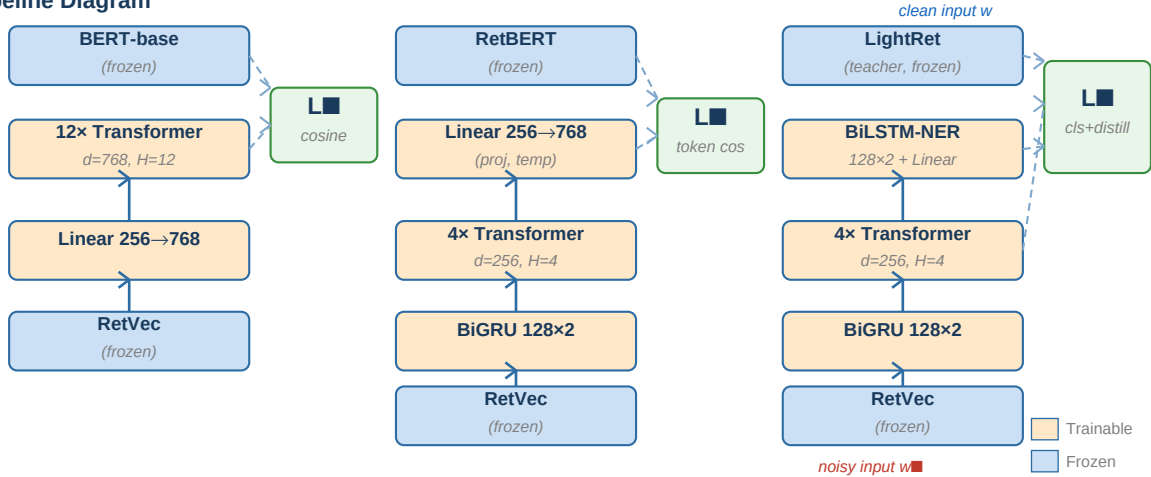
Figure 1: Three-stage LightRet training pipeline. Blue = frozen; Orange = trainable. Stage 3 teacher receives clean input w ; student receives noisy input \tilde{w} .
