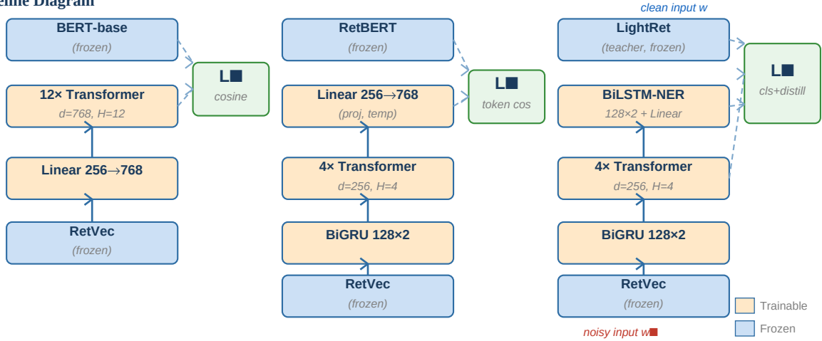
Figure 1: Three-stage LightRet training pipeline. Blue = frozen; Orange = trainable. Stage 3 teacher receives clean input w ; student receives noisy input w .
