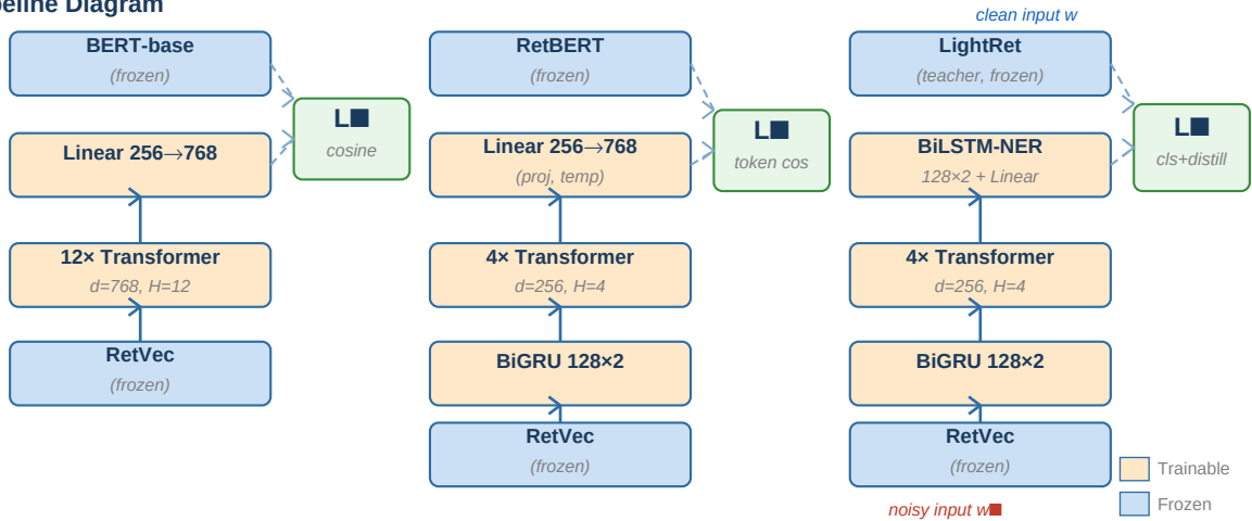
Figure 1: Three-stage LightRet training pipeline. Blue = frozen; Orange = trainable. Stage 3 teacher receives clean input w ; student receives noisy input w\blacksquare .
