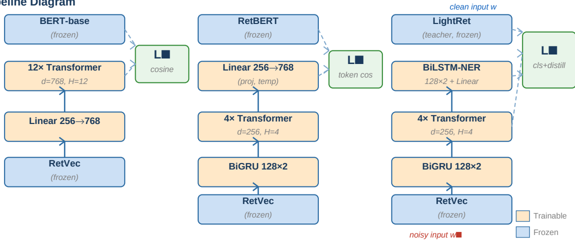
Figure 1: Three-stage LightRet training pipeline. Blue = frozen; Orange = trainable. Stage 3 teacher receives clean input w ; student receives noisy input w_{\sim} .
