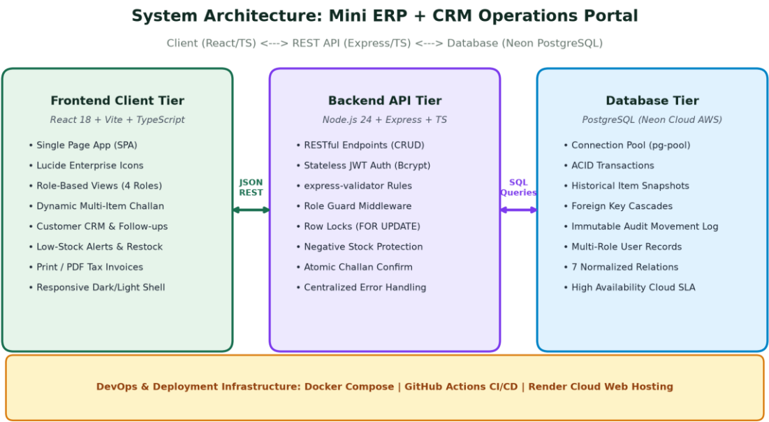
Figure 1: Full-Stack System Architecture (React Frontend, Express API, Neon PostgreSQL DB, and Docker/CI Infrastructure)
