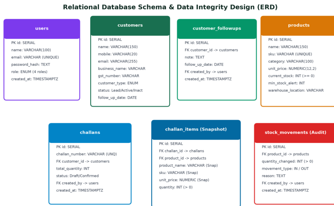
Figure 2: Relational Database Entity Relationship Diagram (ERD) with Constraints & Snapshots
