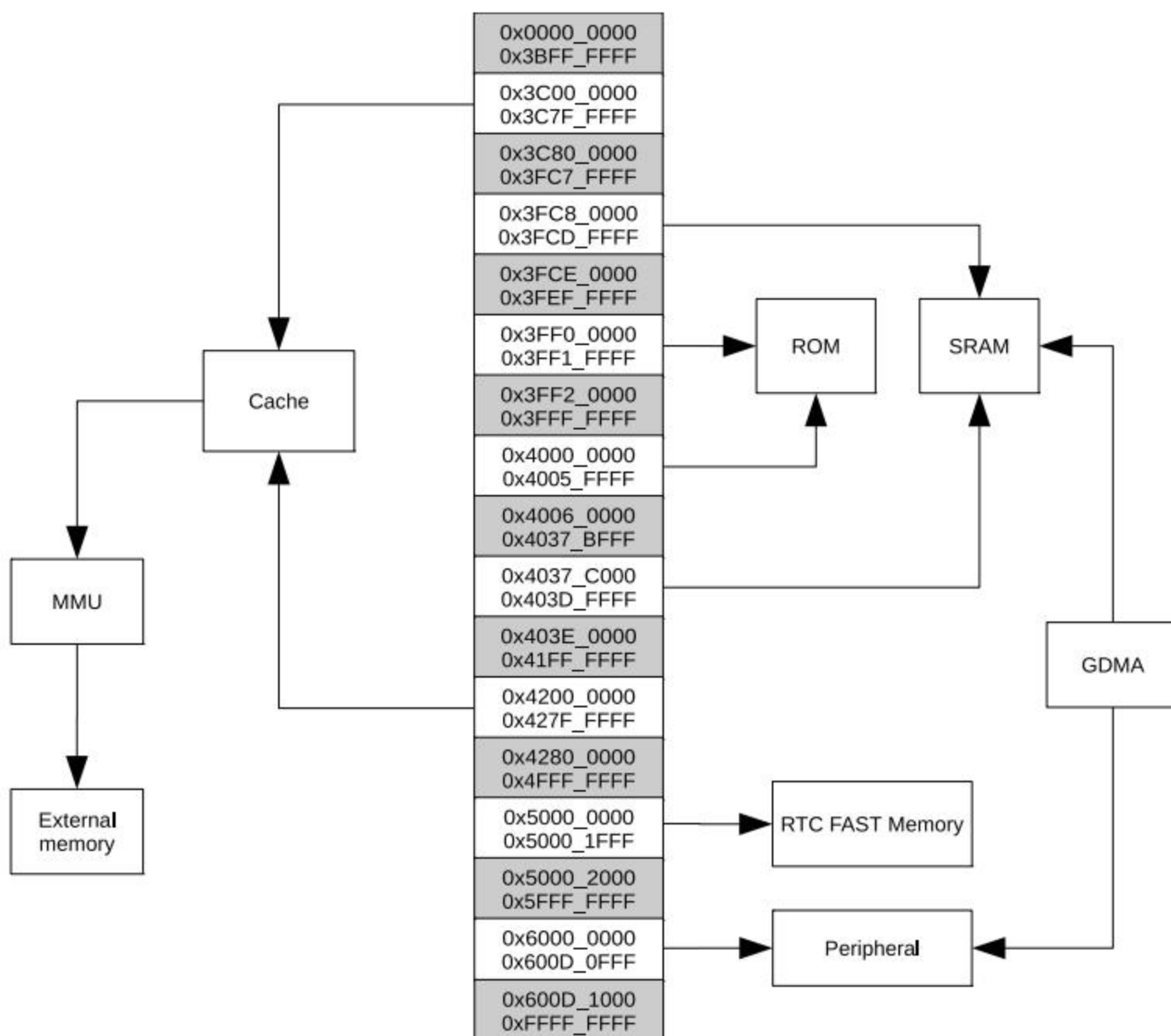
Figure 4-1. Address Mapping Structure
