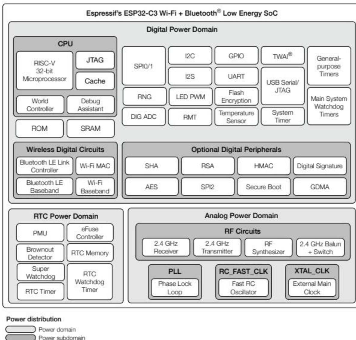
Figure 4-2. Components and Power Domains
