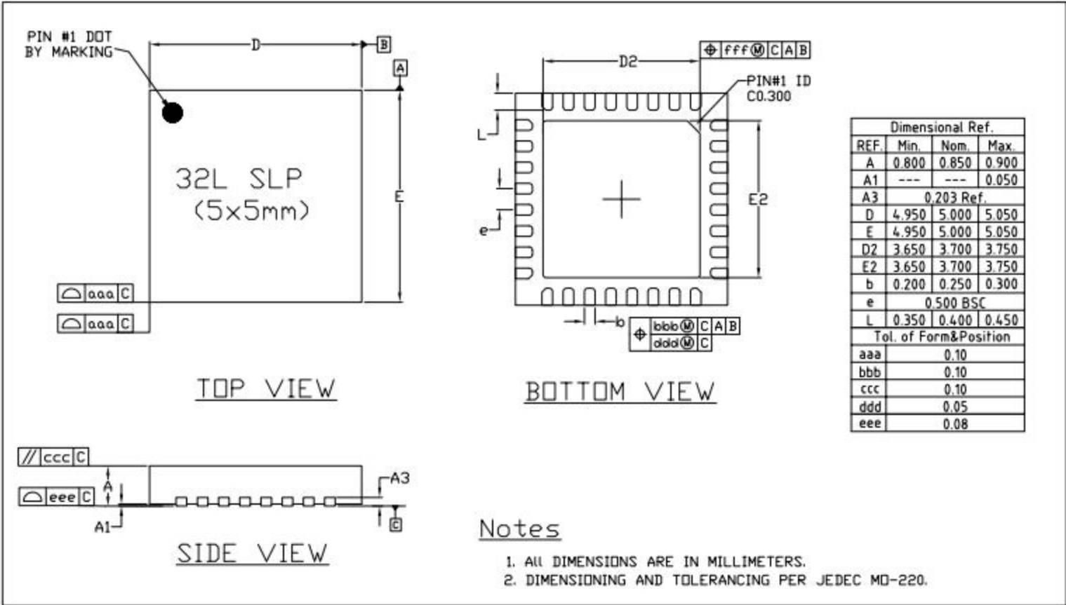
Figure 7-1. QFN32 (5×5 mm) Package
