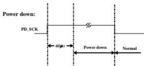
Fig.3 Power down control
