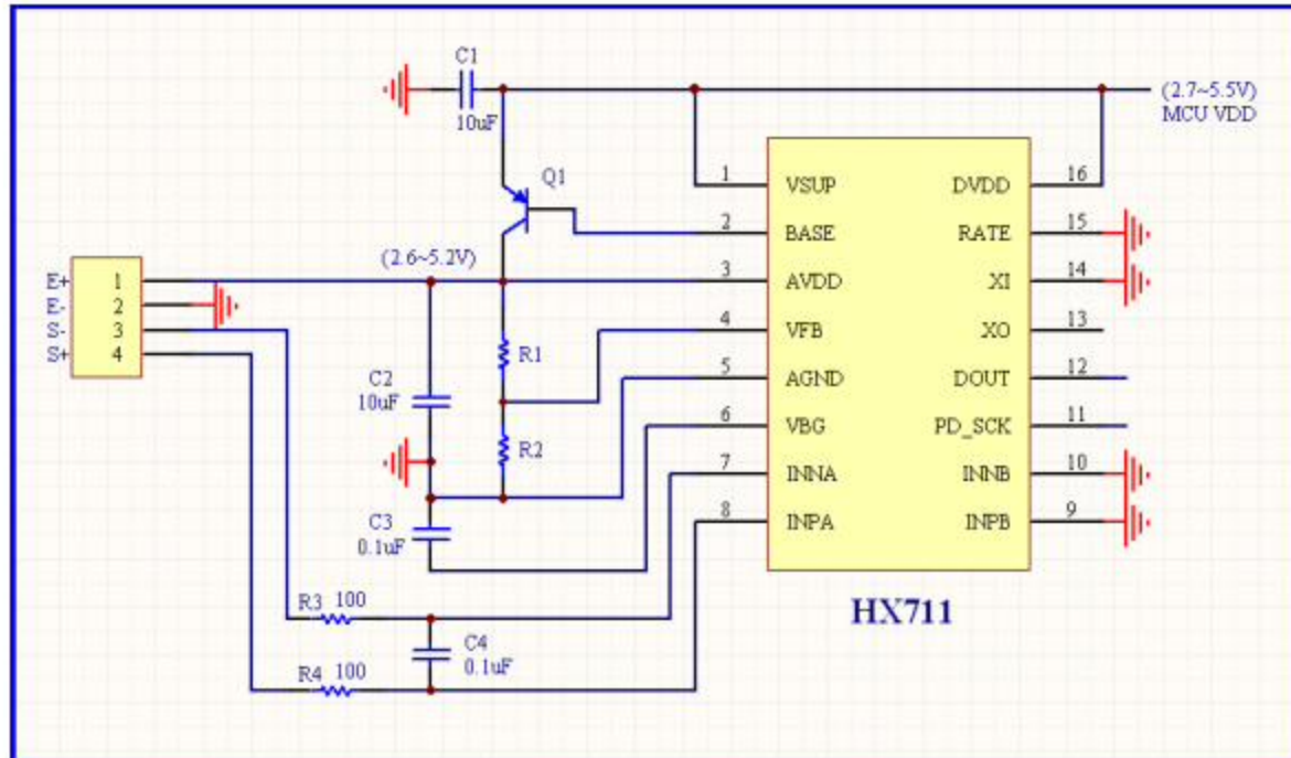
Fig.4 Reference PCB board schematic
