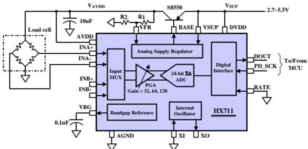
Fig. 1 Typical weigh scale application block diagram
