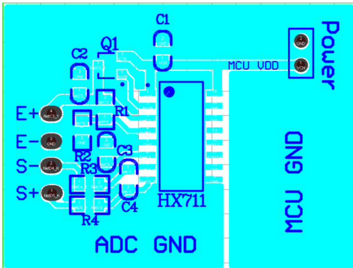
Fig.5 Reference PCB board layout
