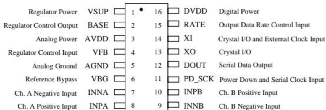
SOP-16L Package
