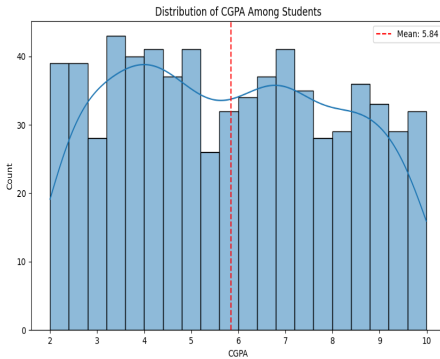
Cgpa Distribution
