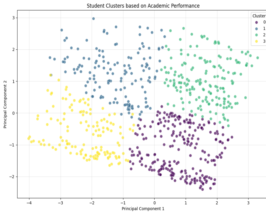
Student Clusters
