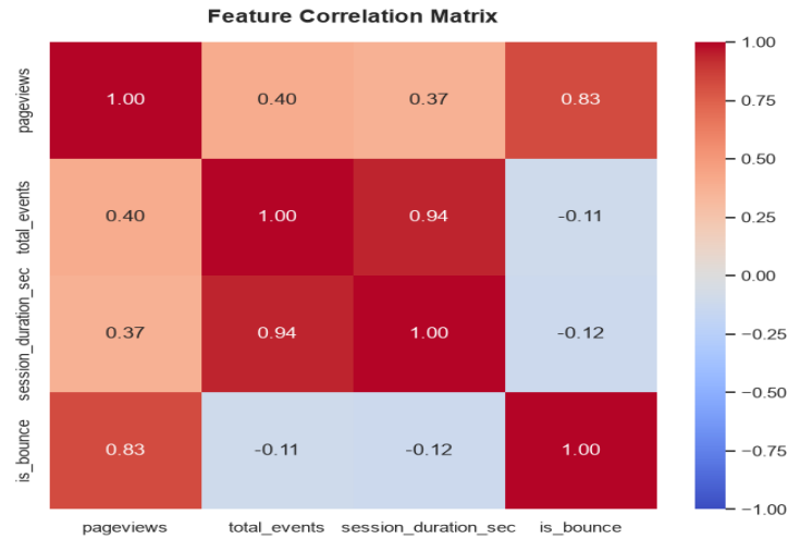
Figure 13: Session Metrics Correlation Heatmap
