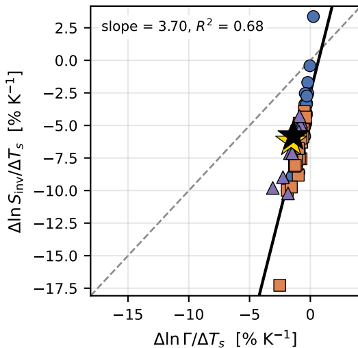
(c) S_{\text{inv}} vs. lapse rate
