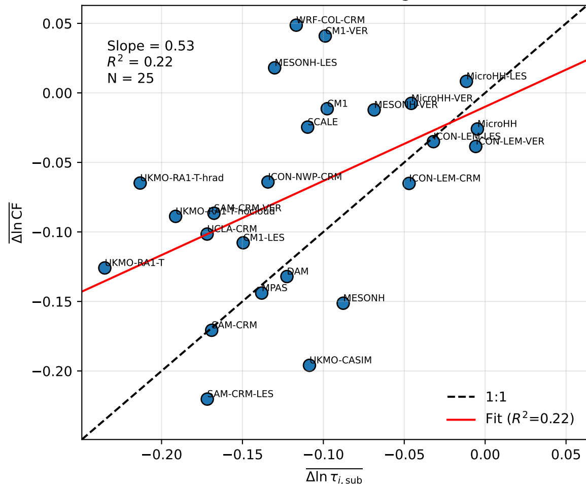
(b) Cloud buffering
