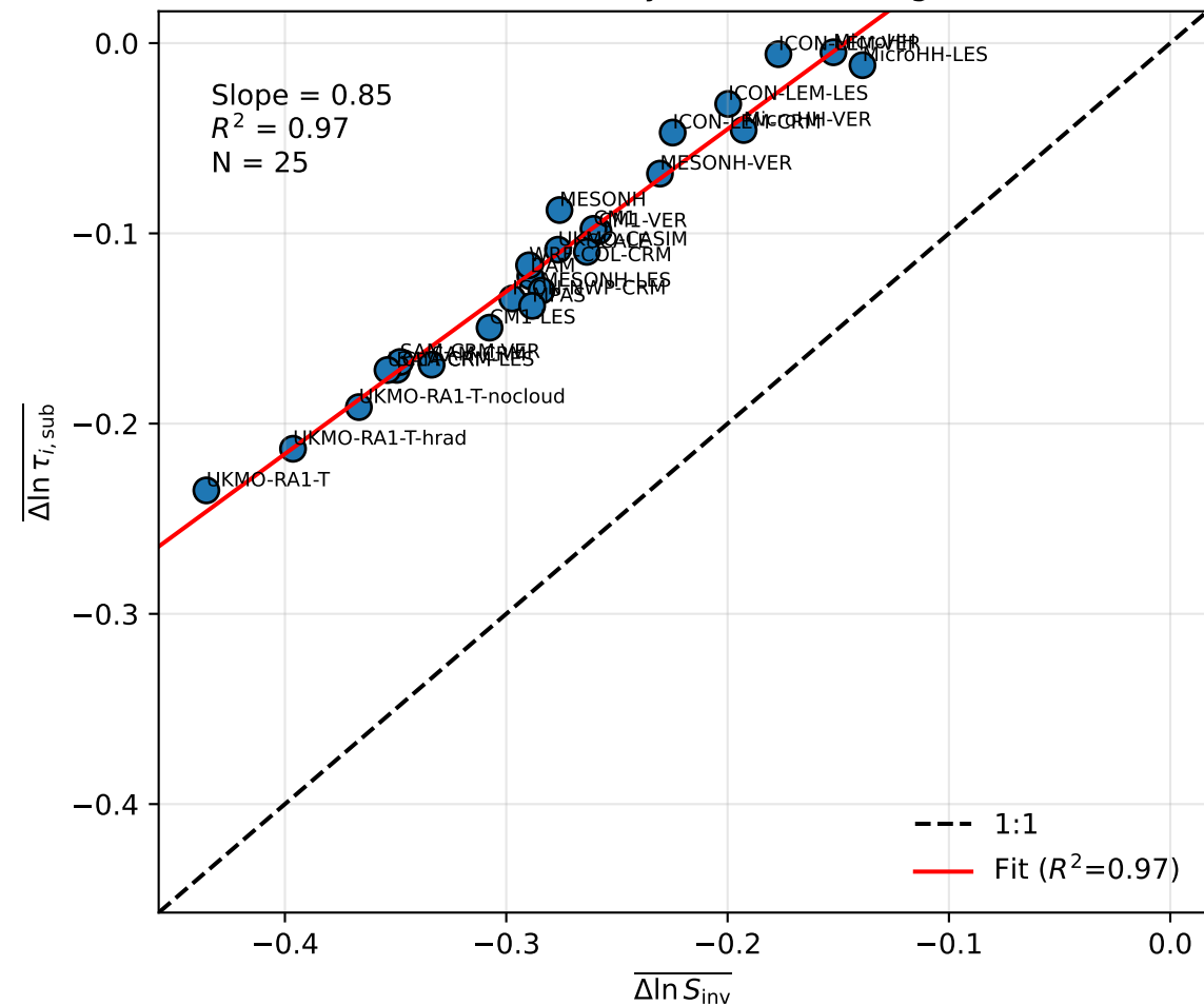
(a) Thermodynamic buffering
