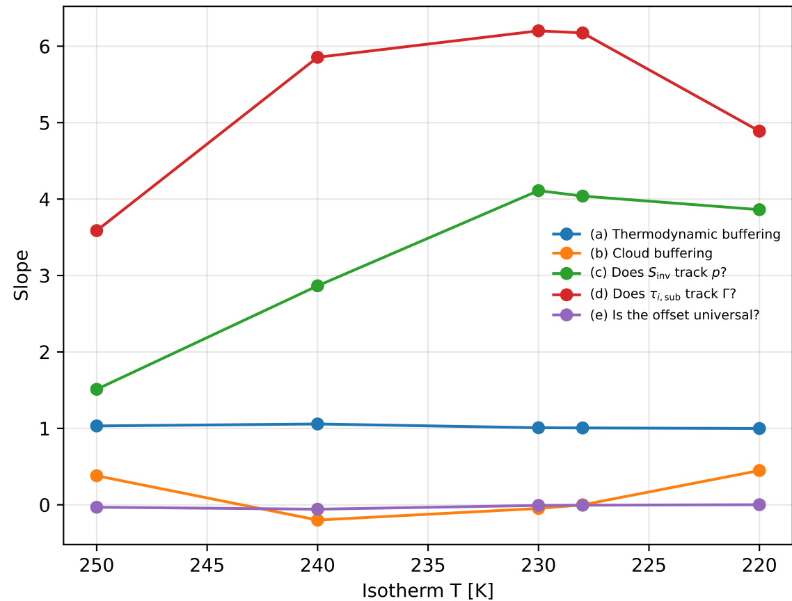
RCEMIP small+large combined, cfv0: sensitivity of the four relationships to isotherm choice Does the slope change with height?
