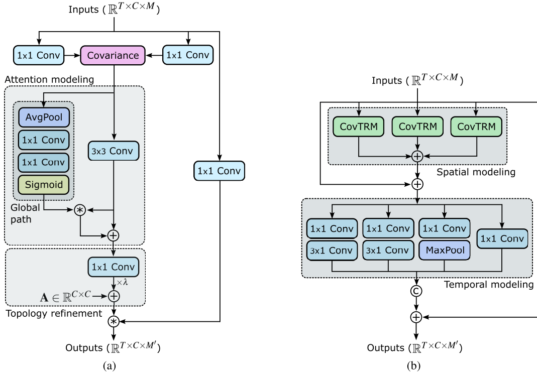
Fig. 2. Proposed modules of CovGCN. For brevity, “Conv” stands for convolution; “MaxPool” stands for max pooling; and “AvgPool” stands for average pooling. (a) CovTRM. (b) GCB.
