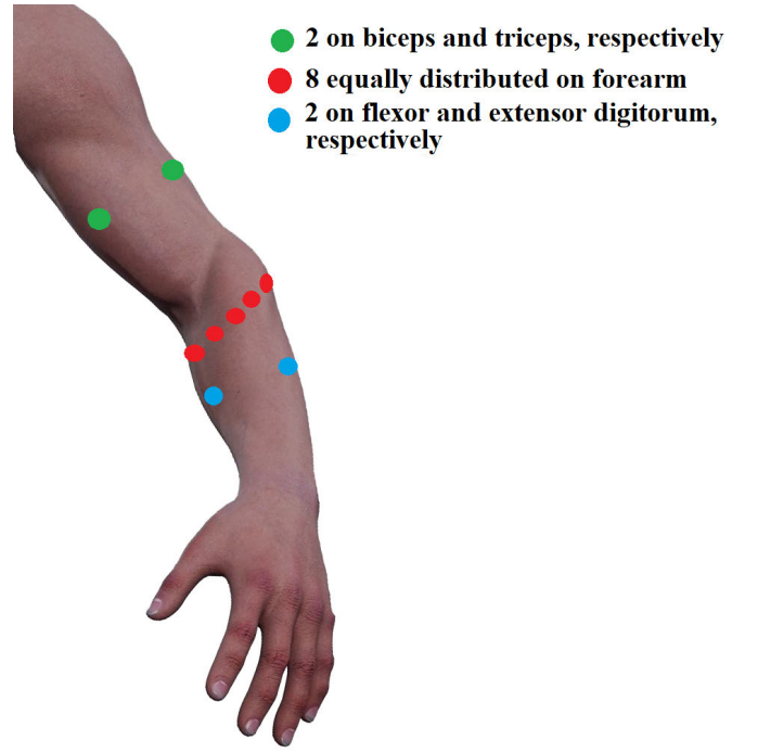
Fig. 3. Placement of 12 sEMG sensors from Ninapro DB2.
