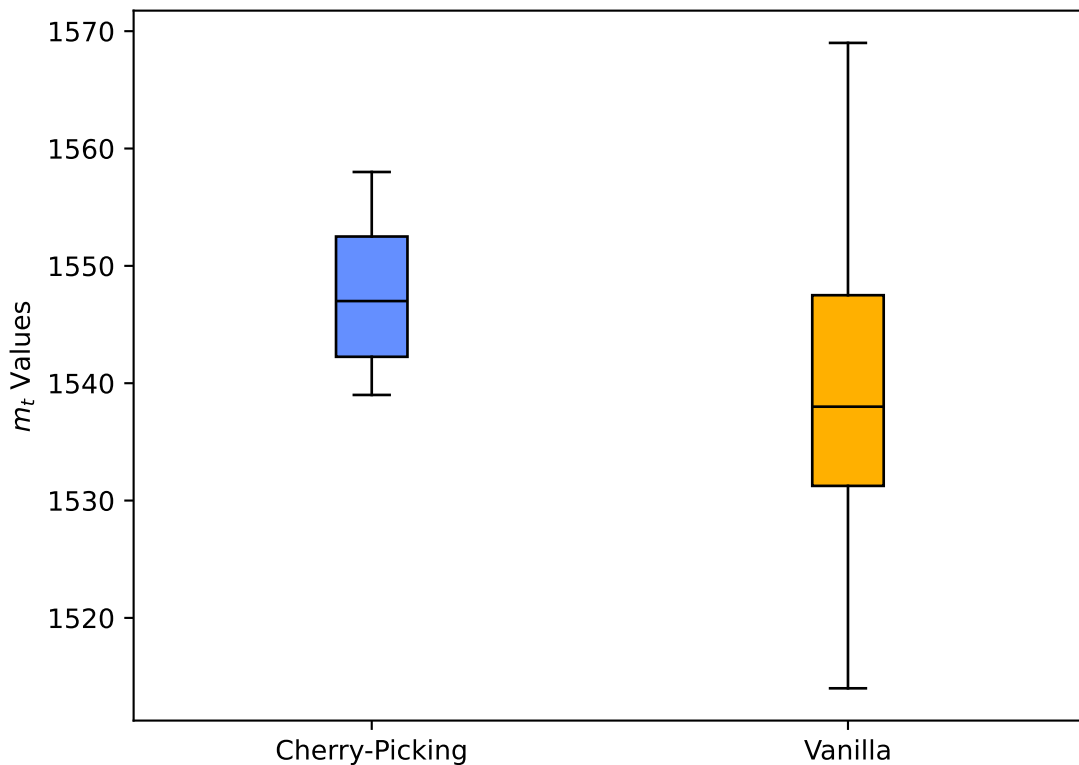
Distribution of m_t Values for Cherry-Picking and Vanilla Tables
