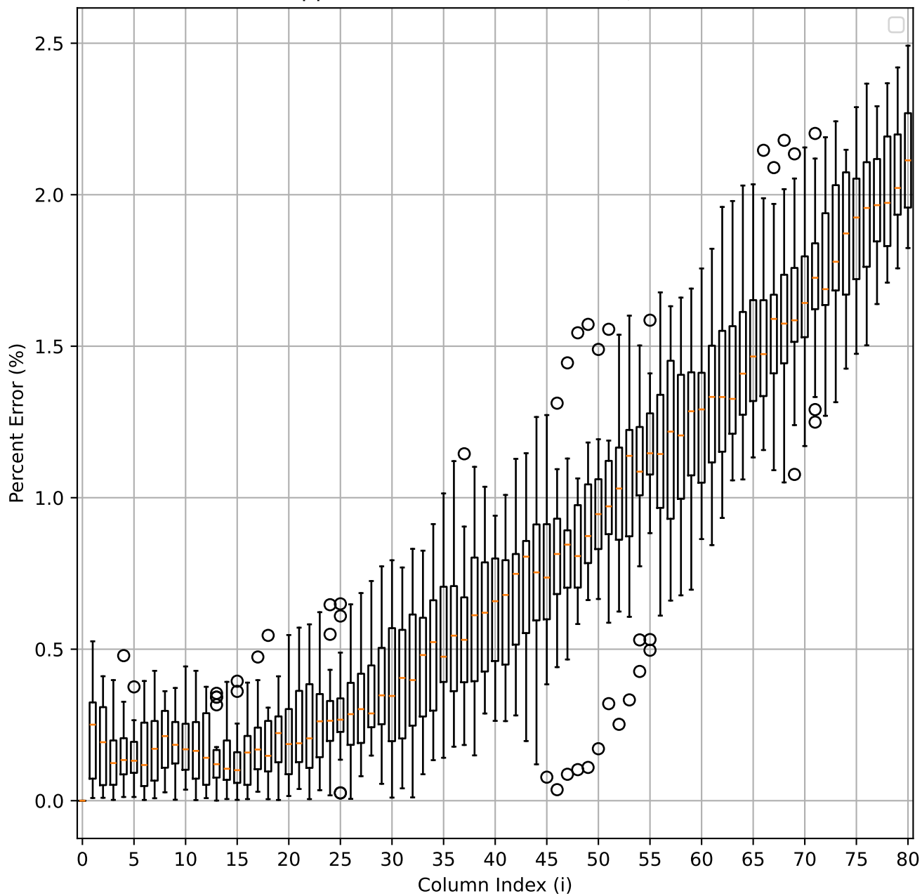
Percent Error of Approximation vs Observed m_i for N=2^{16} and \alpha=0.95
