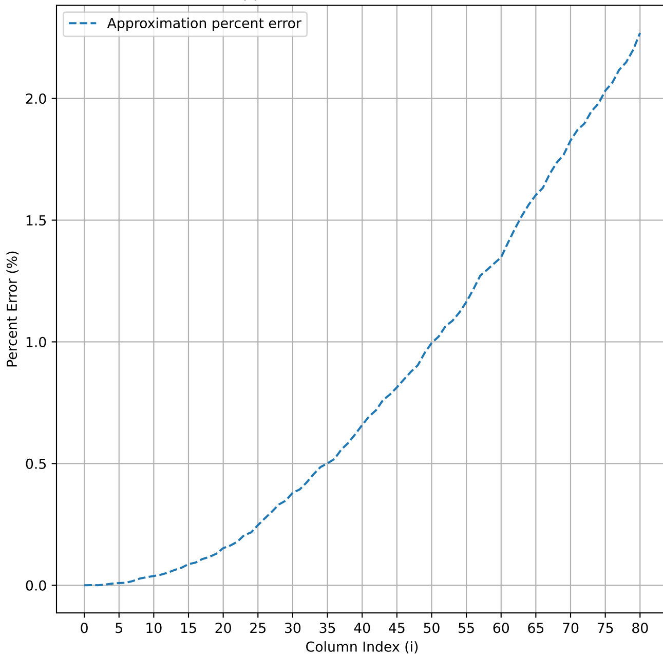
Percent Error of Approximation vs COP m_i for N=2^{16} and \alpha=0.95
