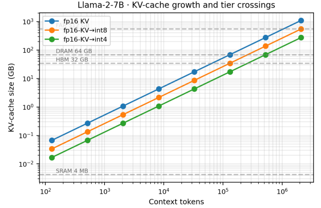
Fig. 5. Llama-2-7B KV-cache size vs. context length under three KV-quant settings. Horizontal dashed lines mark tier capacities. Quantizing fp16 \rightarrow int4 defers each tier crossing by 4\times in context length.
