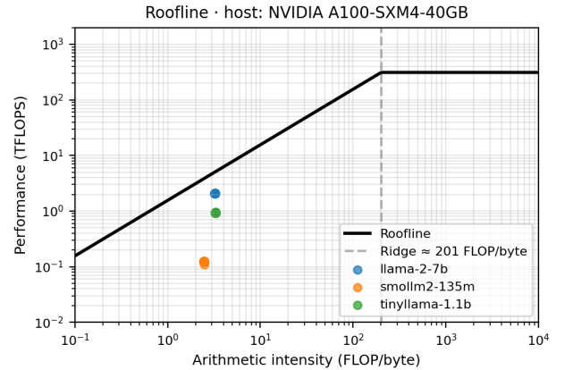
Fig. 2. Roofline against the host A100 GPU. Every measured decode step falls in the memory-bound region by approximately two orders of magnitude. The same clustering holds on T4 (not shown).
