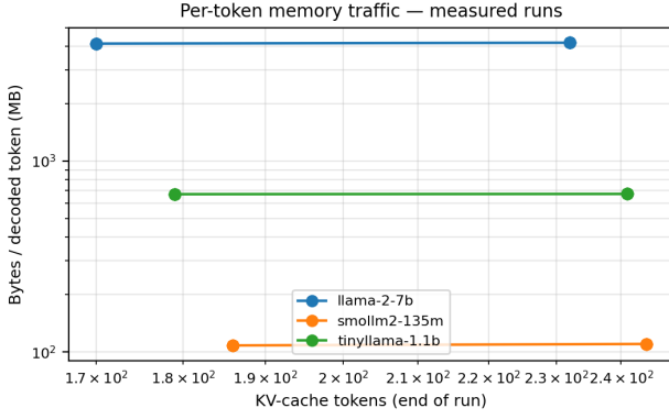
Fig. 6. Per-token memory traffic at decode (real measurements). Curves are dominated by the constant weight term until KV reads catch up; for Llama-2-7B at \text{ctx} = 4096 , KV is still under 7% of total per-token traffic.
