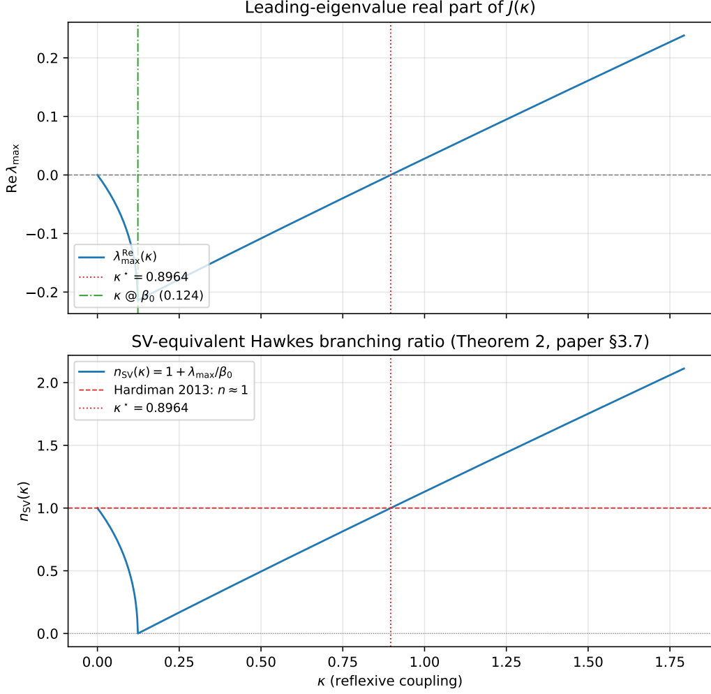
Figure 9: SV-equivalent Hawkes branching ratio n_{SV}(\kappa) at the canonical regime. Top: leading-eigenvalue real part of J(\kappa) , with the gauge zero at \kappa = 0 , the most-stable point at \kappa_{\text{ref}} = 0.124 (the node-spiral transition, \beta_0 \approx 0.214 ), and the Hopf threshold \kappa^* = 0.8964 where \lambda_{\max} = 0 . Bottom: n_{SV}(\kappa) = 1 + \lambda_{\max}/\beta_0 , anchored by n_{SV}(\kappa_4^*) = 0.99996 \approx 1 where the residual 4 \times 10^{-5} is the truncation error in the 4-decimal \kappa_4^* = 0.8964 ; at machine-precision \kappa^* the identity is exact (Theorem 2, claim 1); the empirical Hardiman et al. (2013) n \approx 1 is the dashed red line. Past \kappa^* , n_{SV} > 1 (Hawkes-non-stationary regime). Run dir: runs/hawkes_sv_equivalence/ .
