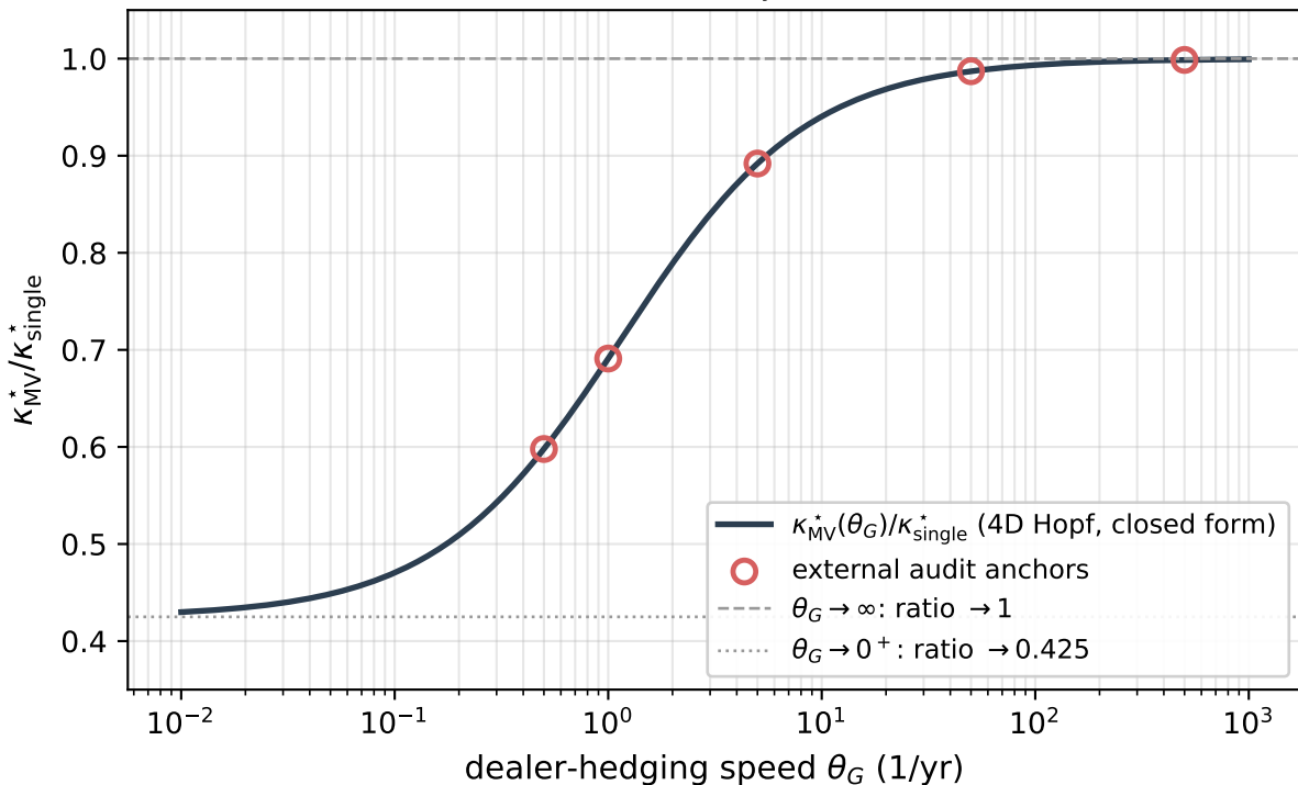
Corrected MV Hopf-threshold ratio (v0.3.6) Canonical short-gamma regime (G_y, G_v, G_z) = (1/2, -1/2, -1/2)
