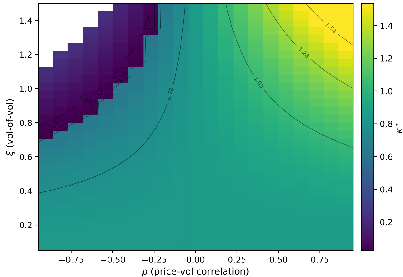
\kappa^*(\xi, \rho) at \sigma_v = 0.50
