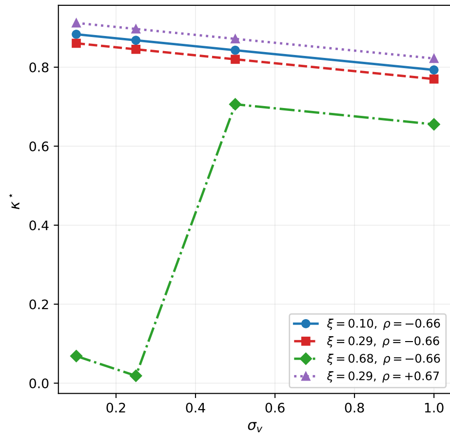
\kappa^*(\sigma_v) at representative (\xi, \rho)
