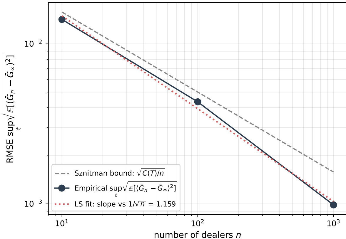
Propagation-of-chaos for the dealer-gamma channel (McKean-Vlasov mean-field SDE; canonical \sigma_q = 0.10 regime)
