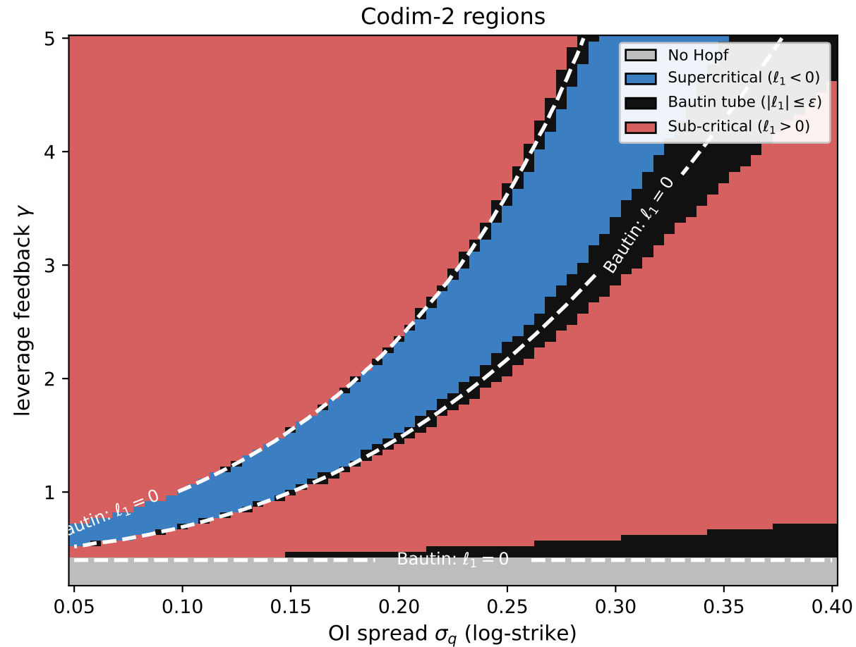
Codim-2 bifurcation structure in (\sigma_q, \gamma) at canonical (\alpha, \kappa_v, T_{\text{eff}}, \beta) = (0.05, 2, 0.25, 1)
